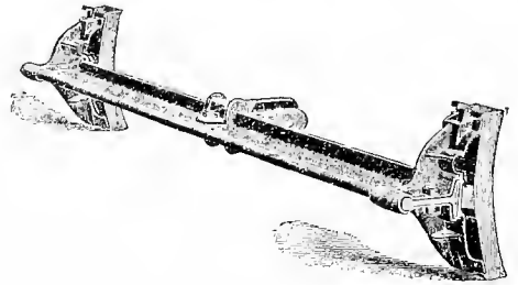
Fig. 1600. THE MARDEN BRAKE-BEAM, WEIGHT 87 LBS., MADE BY MARDEN CAR BRAKE COMPANY.
